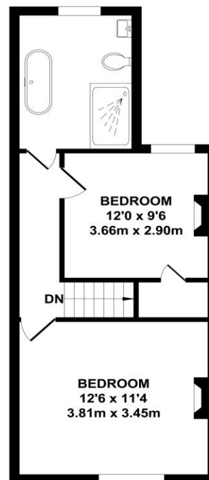
FIRST FLOOR APPROX. FLOOR AREA 377 SQ.FT. (35.01 SQ.M.)
